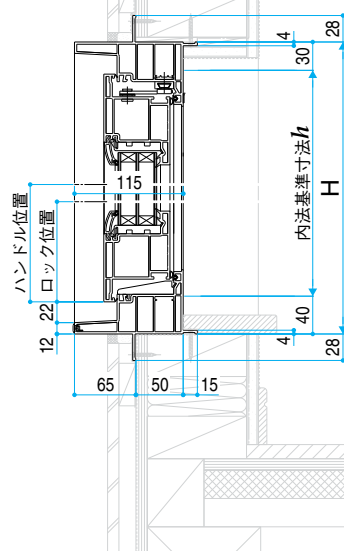
●2連窓
