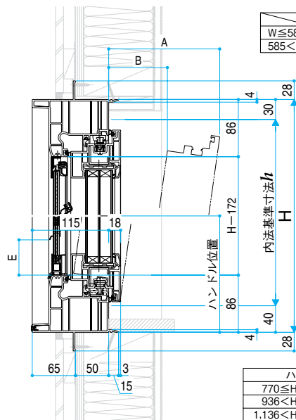
●段窓
