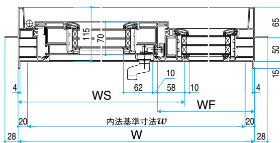
●2連窓
