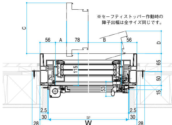
●段窓
